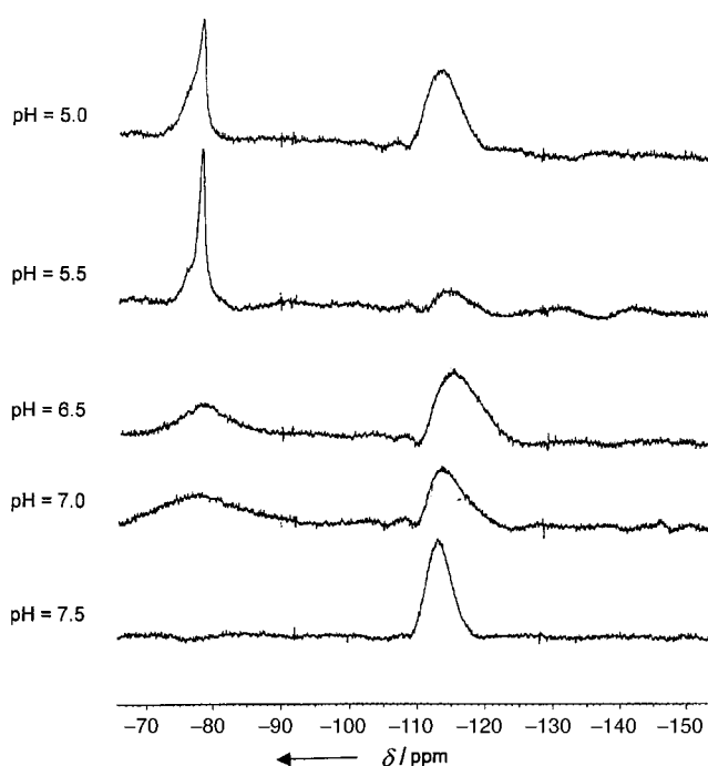
Figure 4. ^{19}\text{F} NMR spectra of NaF:PEAcryp·6Ts (10 mM) in 0.1 M KT at -25^\circ\text{C} in \text{DMSO}:\text{H}_2\text{O} (40:60).
